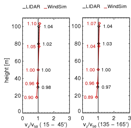
Fig. 6: Comparison of vertical wind speed profiles from WindSim and LIDAR data normalised to 50 m for the wind directions north-north-east (left) and south-south-east (right).
