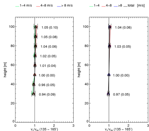
Fig. 5: Vertical wind speed profiles from SODAR (left) and LIDAR (right) normalised to 50 m for the wind direction south-south-east, in brackets the standard deviations.
