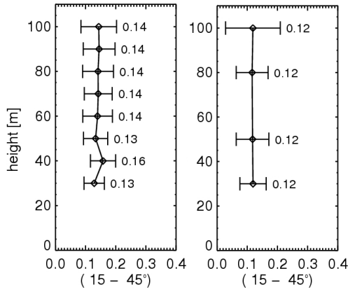
Fig. 7: Comparison of vertical turbulence intensity profiles from SODAR (left) and LIDAR (right) data for the wind direction north north-east. The bars indicate the standard deviation.
