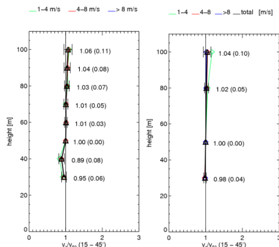
Fig. 4: Vertical wind speed profiles from SODAR (left) and LIDAR (right) normalised to 50 m for the wind direction north-north-east, in brackets the standard deviations.
