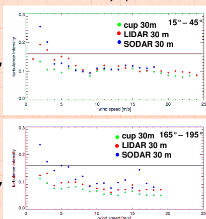
Fig. 6: Turbulence intensity of cup data (green), LIDAR data (red) and SODAR data (blue) at the height of 30 m for the sector 15°-45° (top) and 165°-195° (bottom).
