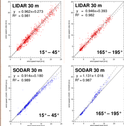
Fig. 3: Scatterplot of 30 m wind speed: cup – LIDAR (red) and cup – SODAR (blue), for the wind sectors 15-45° (left) and 165-195° (right).
